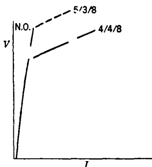
FIG. 8-24.—A steady-state characteristic of the LM2. At high voltages the \frac{3}{2} -component is excited at the start of each pulse.
